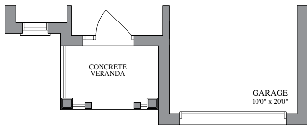
FIRST FLOOR ELEVATION B
