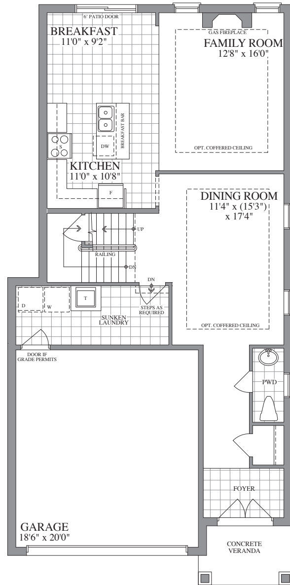
FIRST FLOOR ELEVATION A & B
